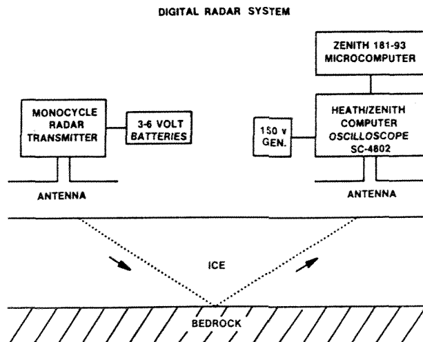
Fig. 2. Block diagram of an ice-radar system including the PC-based receiver.
