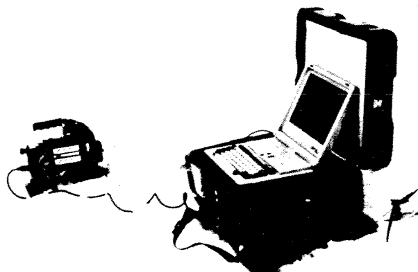
Fig. 1. The PC-based ice-radar receiver in operation on Mount Estelle glacier, Alaska, U.S.A.
