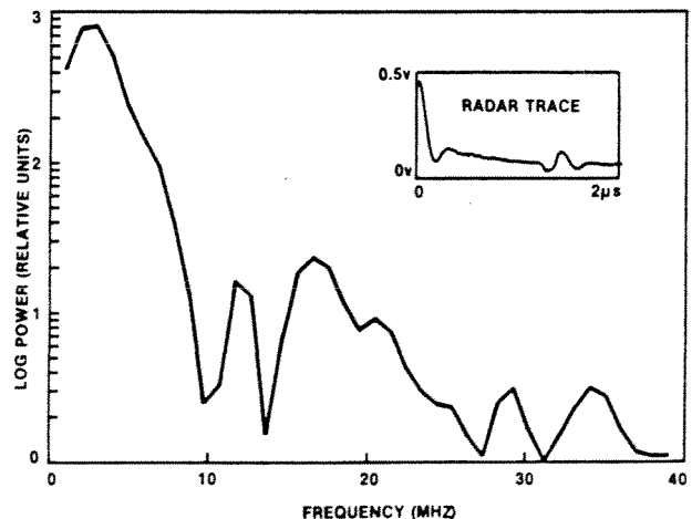
Fig. 3. A typical digital wave form recorded on Mount Estelle glacier, Alaska, and its power spectrum. The PC-based receiver allows the use of a wide variety of standard signal-analysis software in the field.
