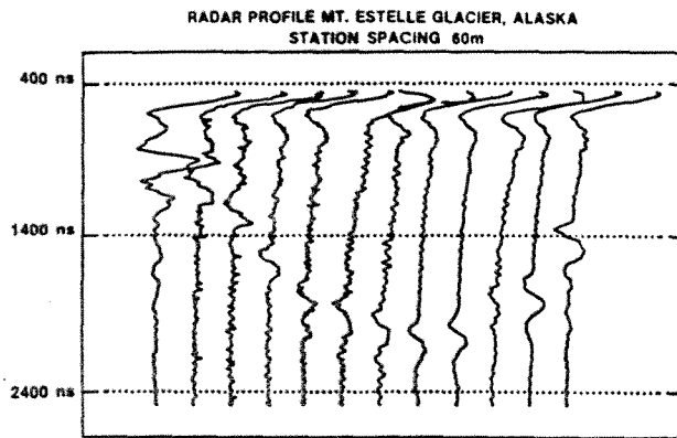
Fig. 4. An ice-radar profile across Mount Estelle glacier as recorded using the PC-based receiver.
