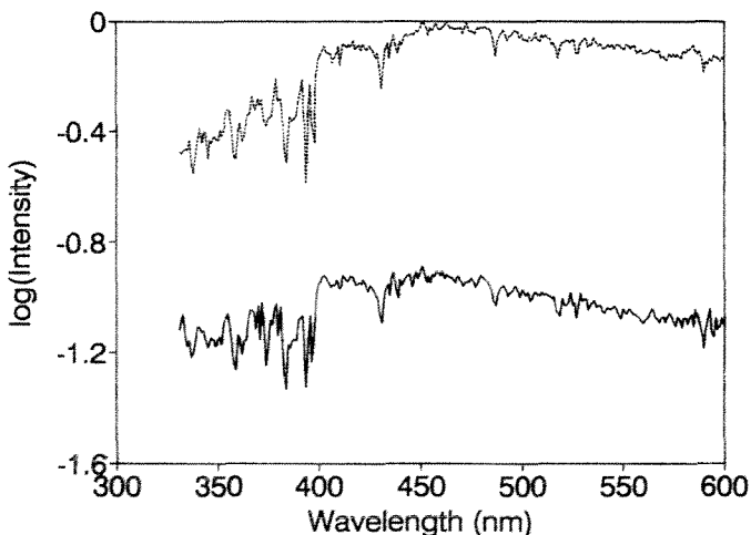
Fig. 3: Microamperes ( I ) from the light detector for measurements of downward sky spectral radiance under clear (solid line) and cloudy (dotted line) conditions. The light was collected by pointing the optic cable end straight up ( 12^\circ field of view). The solar elevations were 46^\circ and 44^\circ respectively.
