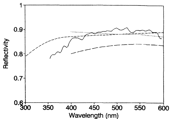
Fig. 5: The solid line is the spectral reflectivity of snow taken on the Taku Glacier, 27 July 1991. Note that the reflectivity has its maximum in the blue-green, and decreases both for longer and shorter wavelength. The dotted line is a measured spectrum by GRENFELL & MAYKUT (1977) carried out near T-3 in the Arctic Ocean, the shorter dashed line is from model calculations by WARREN (1982) for snow with a volcanic ash concentration of 10 ppm by weight, and the long dashed line is alpine snow from GRENFELL & PEROVICH (1981).
