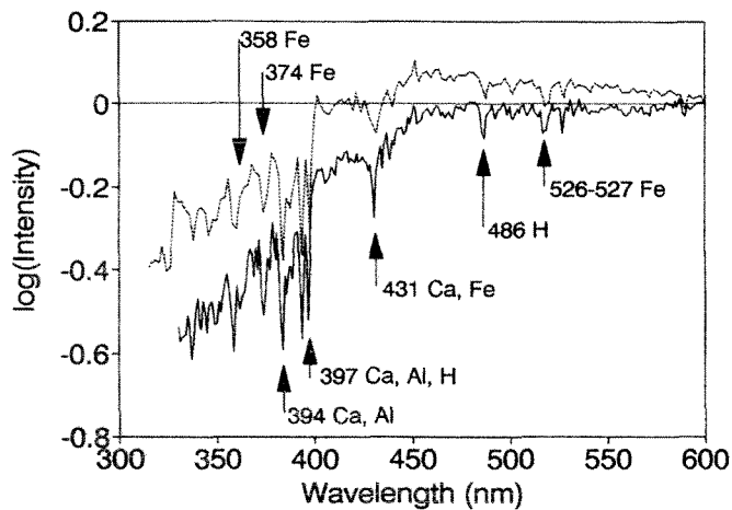
Fig. 2: The solid line is a direct beam spectral irradiance ( F ) measured at 10:45, 21 July 1991 solar time (solar elevation = 45^\circ ), on the Taku Glacier, Juneau Icefield, Alaska. The cable end was aimed at the sun under clear sky conditions. The dotted line is the direct beam spectral irradiance ( F ) above the Earth's atmosphere as reported by IQBAL (1983). Each curve has been normalized to the irradiance at 600 nm ( F_0 ).
