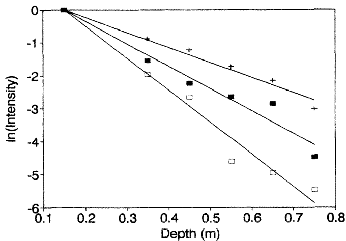
Fig. 6: The natural log of the light detector current for measurements of radiance in different wavelength bands vs. snow depth. For totally uniform snow, a straight line is expected. The symbols are: Filled square = 350-370 nm, plus = 450-470 nm, and empty square = 590-610 nm. The 590-610 nm (red) band shows the strongest decrease with depth, while 450-470 nm (blue) is absorbed the least. 350-370 (UV) lies between these two values. The 520-540 nm band (green, which is not shown) displayed very similar values to the UV.
