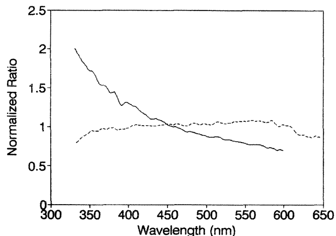
Fig. 4: Downward spectral radiance ratios. The solid line is the clear sky diffuse radiance divided by the clear sky direct beam. The dotted line is the downward diffuse radiance measured under a thick stratus cloud layer divided by the same direct beam measurement. Both curves are normalized at 450 nm. The clear sky and direct solar beam measurements were taken near 11:00, 21 July 1991 solar time (solar elevations = 46^\circ and 44^\circ respectively), and the cloudy sky measurement was taken at 10:44, 27 July 1991 solar time (solar elevation = 43^\circ ). The sky radiance measurements were taken by pointing the optic cable end straight up ( 12^\circ field of view).
