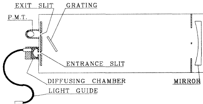
Fig. 1: Schematic of the spectrometer optics with synthetic quartz fiber optic light guide, entrance light diffuser, and photomultiplier tube (PMT) detector.
