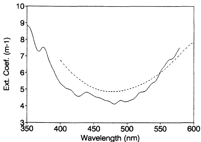
Fig. 7: The solid curve is the extinction coefficient in snow on Taku Glacier, 26 July 1991. The dotted curve is from model calculations for pure snow with a snow grain size of 1.3 mm (WARREN 1982)
