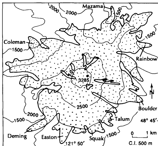
Figure 2. Glaciers on Mount Baker that have been part of the NCGCP study. See data in Table 1.
