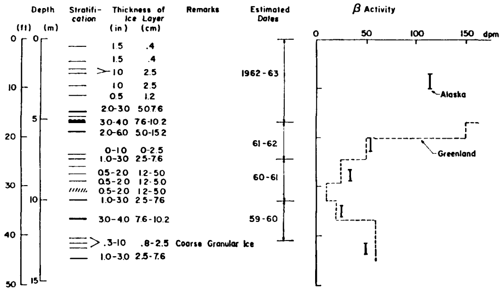
Fig. 2. Firm stratigraphy and \beta activity, site 8, Juneau Icefield
