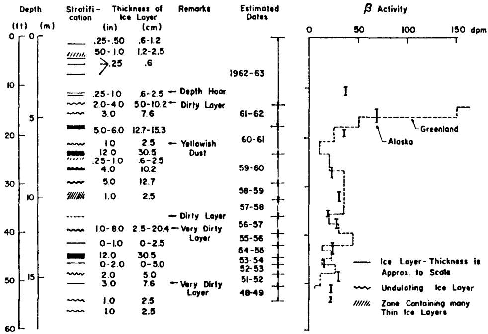
Fig. 1. Firm stratigraphy and \beta activity, site 10, Juneau Icefield
