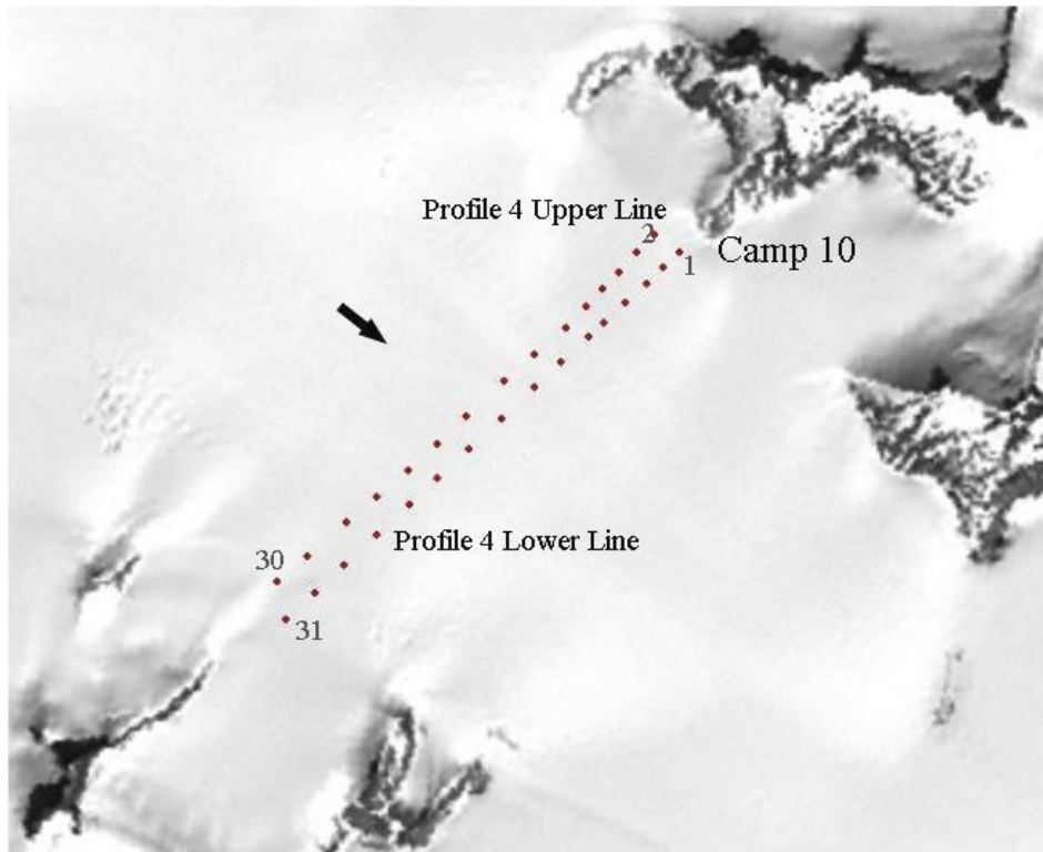
Figure 2. Position of marker flags on Profile IV for the upper and lower line. Flow direction noted by arrow. Base Station is on nunatak at Camp 10. Selected flag numbers listed.
