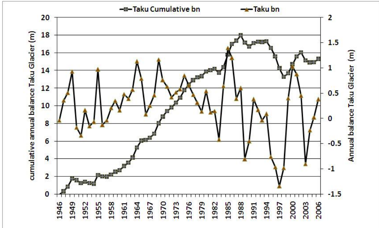
Figure 3. Annual and cumulative mass balance of the Taku Glacier 1946-2006.
